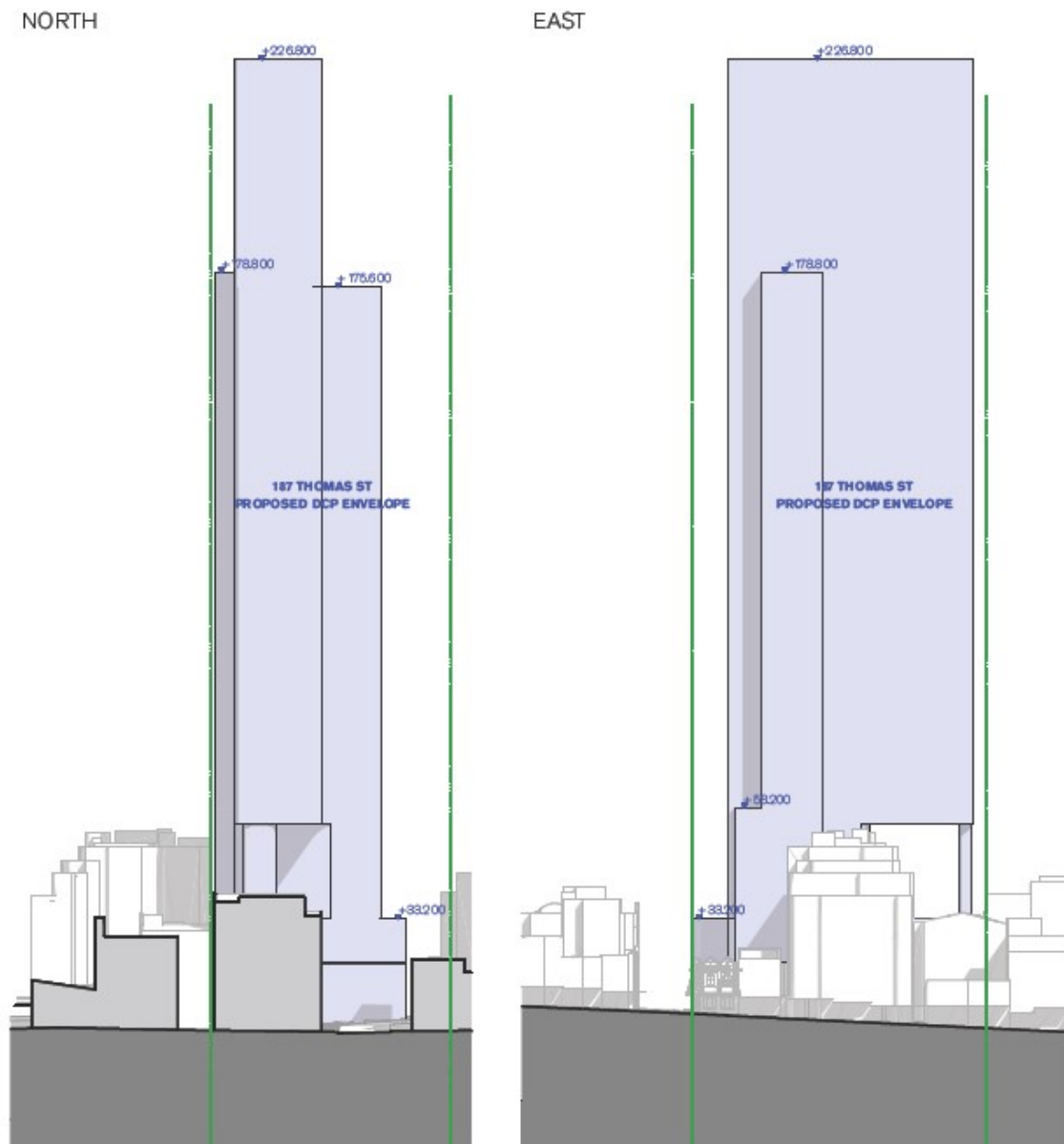
Figure 6.X North and East Envelope Elevations (Source: FJMT, March 2020)
